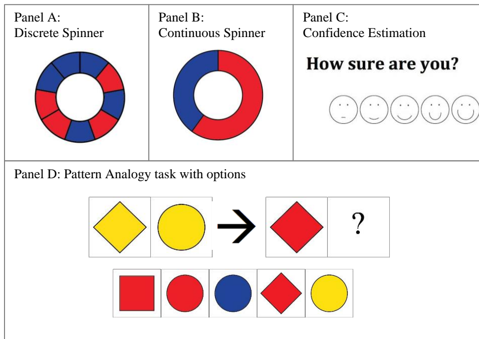
Figure 1: Example Stimuli
